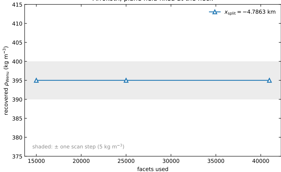
Arrokoth, plane held fixed at the neck
