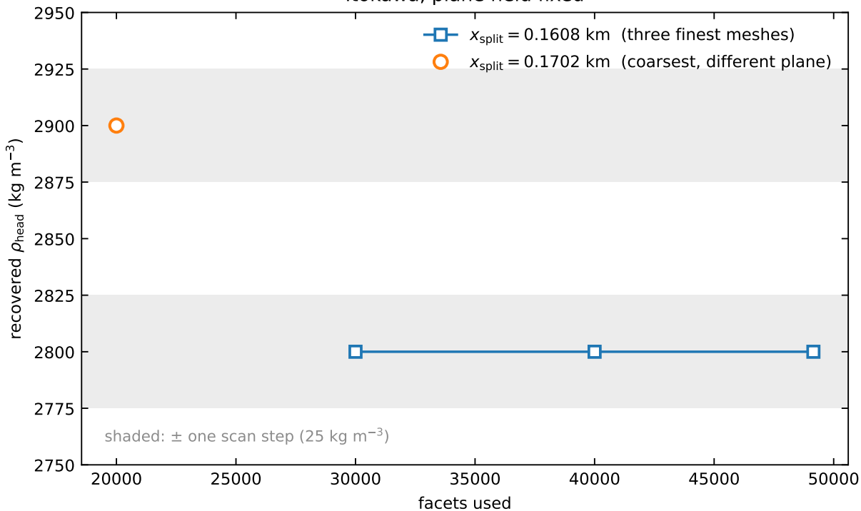
Itokawa, plane held fixed
