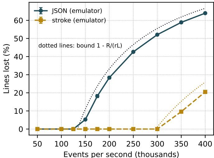
(a) Loss, 90 s run, R = 32 MB/s
