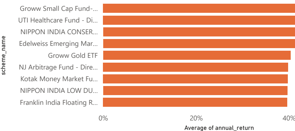
Average of annual_return by scheme_name
