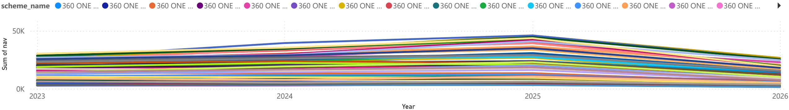
Sum of nav by Year and scheme_name
