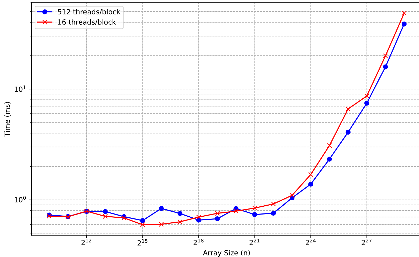
Task 3: Vscale Execution Time vs Array Size
