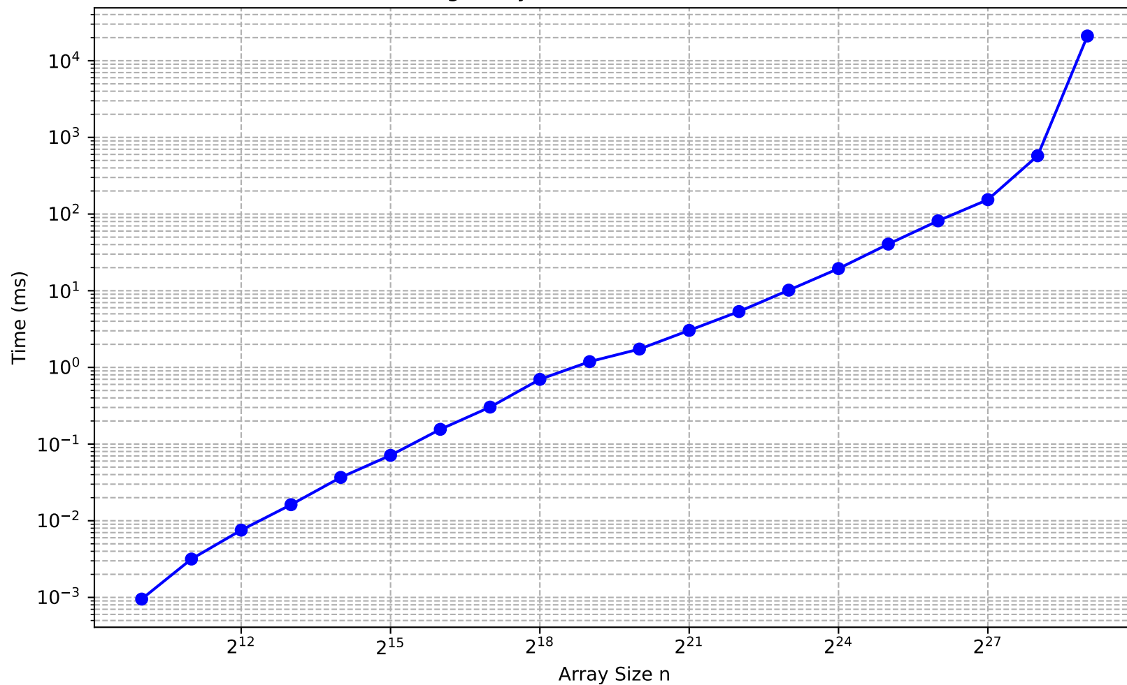
Scaling Analysis of Inclusive Scan (Task 1)
