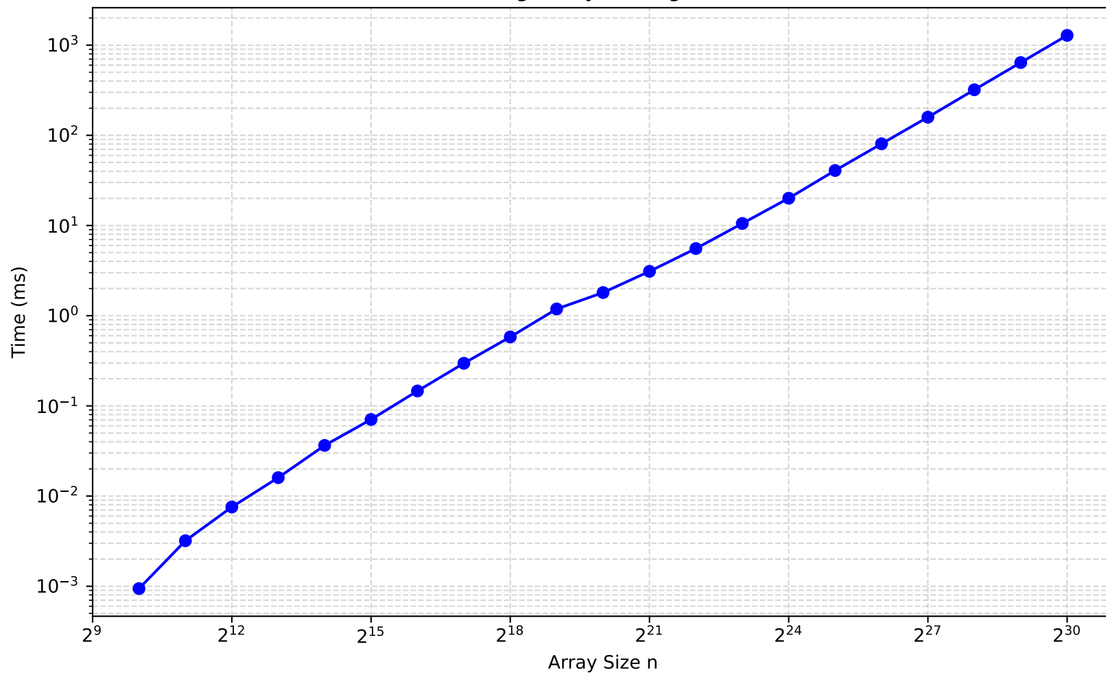
Scaling Analysis (Log Scale)
