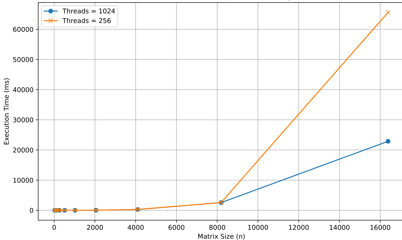
Task 1: Matrix Multiplication Scaling
