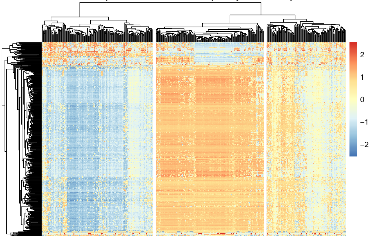
Top 500 Variable Probes (Methylation, k=3 )
