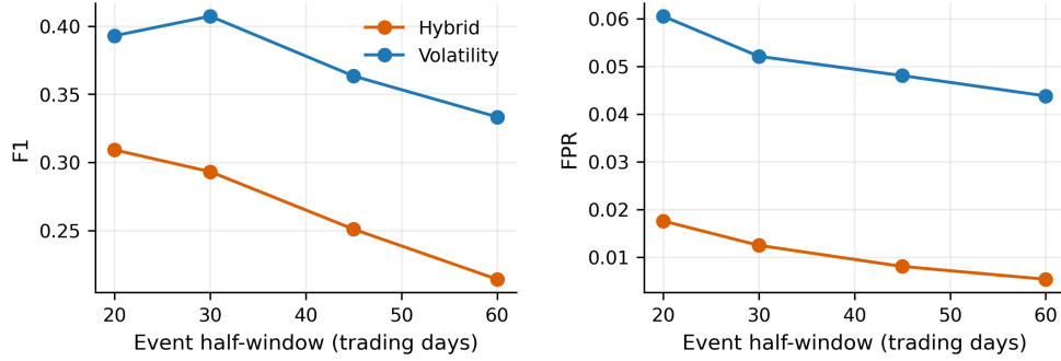
Fig. 5 Event-window sensitivity across \pm 20 , \pm 30 , \pm 45 , and \pm 60 trading-day windows.
