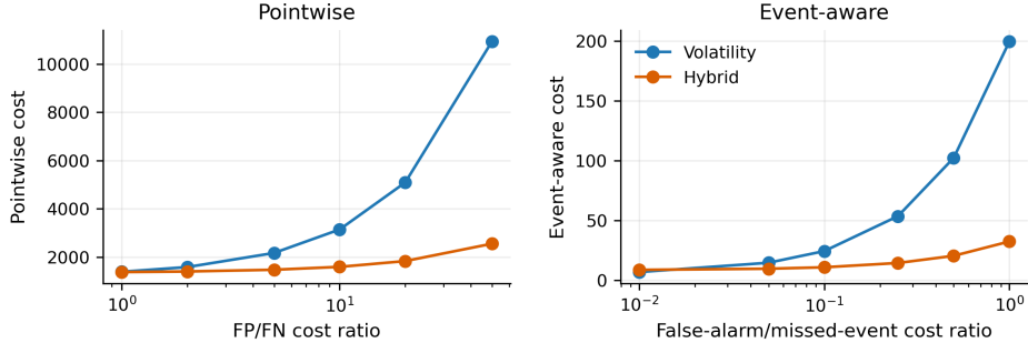
Fig. 4 SPY cost comparison under pointwise and event-aware operating objectives.
