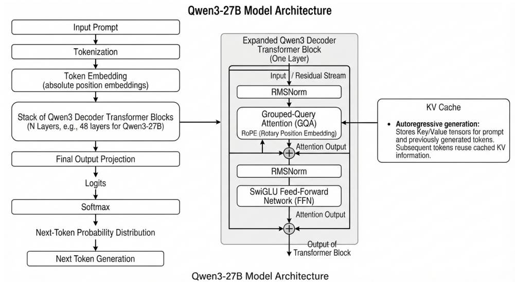
Figure 9-2. Qwen3-style decoder-only Transformer with GQA, RoPE, SwiGLU, and RMSNorm
