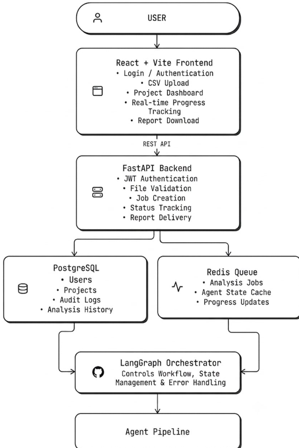
Figure 5.1: System architecture and agent flow
