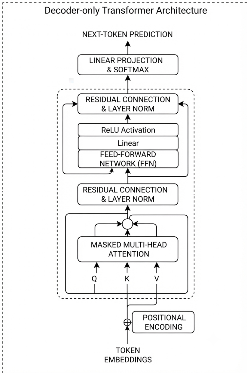
Figure 4.1: Decoder-only Transformer architecture used by modern LLMs
