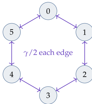
The 6-director rotation graph. Each edge represents both m \rightarrow m \pm 1 at rate \gamma/2 ; total rate \gamma out of each node.
