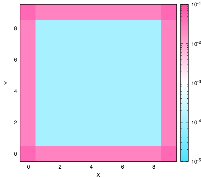
\omega = 0.5 (achiral)
