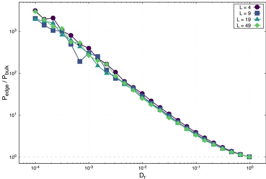
TCRW Fig 3(a) — edge localization vs D_r ( \omega = 1 , T = \max(10^8, 100 \cdot \max(L^2, 1/D_r)/D_r) )
