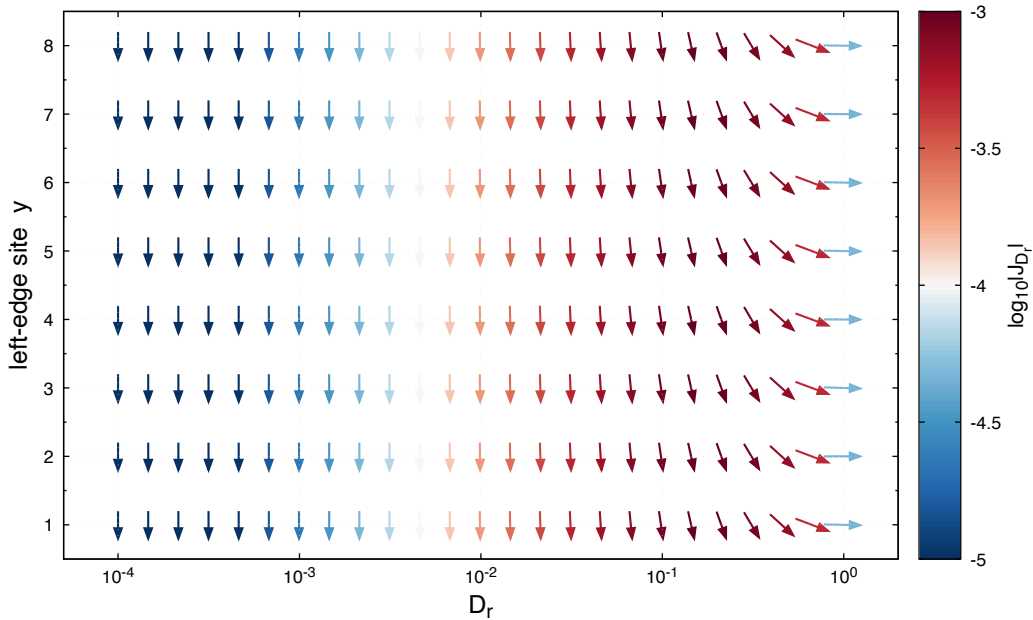
TCRW Fig 3(c) — J_{D_r}(y) on left wall ( L = 10 , \omega = 1 )
