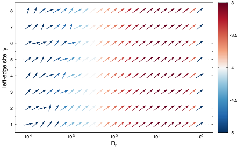
TCRW Fig 3(d) — J_\omega(y) on left wall ( L = 10 , \omega = 1 )
