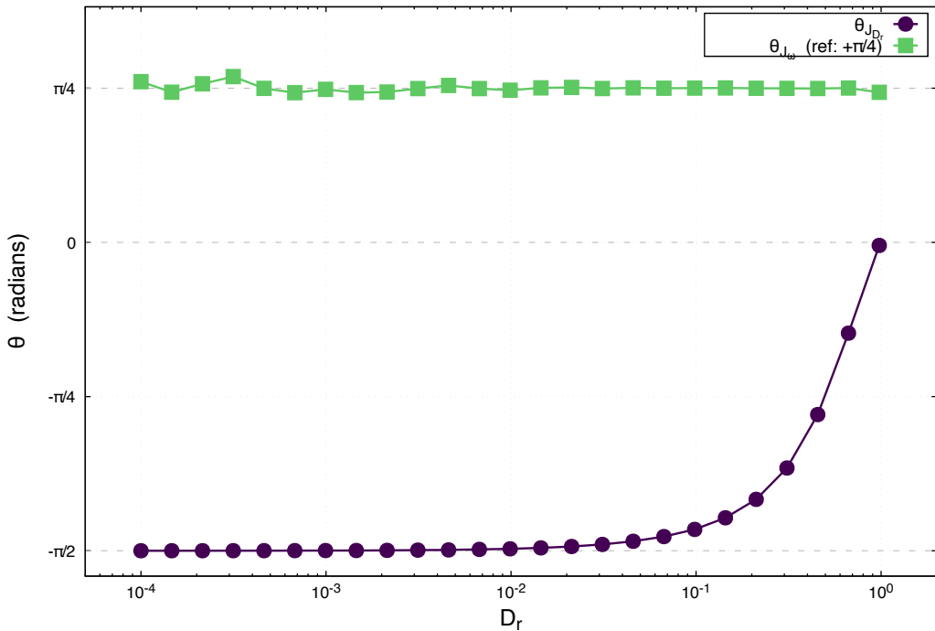
TCRW Fig 3(e) — \theta of total left-wall currents vs D_r ( L = 10 , \omega = 1 )
