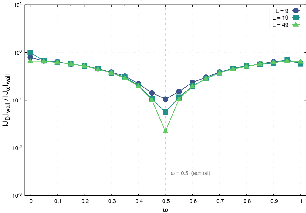
TCRW Fig 3(g) — |J_{D_r}|/|J_\omega| on left wall vs \omega ( D_r = 10^{-3} , OBC)
