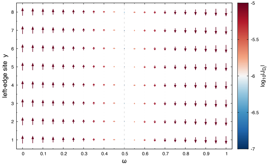
TCRW Fig 3(h) — J_{D_r}(y) on left wall ( L = 10 , D_r = 10^{-3} )
