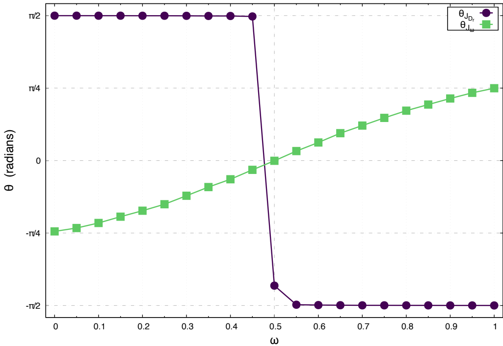
TCRW Fig 3(j) — \theta of total left-wall currents vs \omega ( L = 10 , D_r = 10^{-3} )
