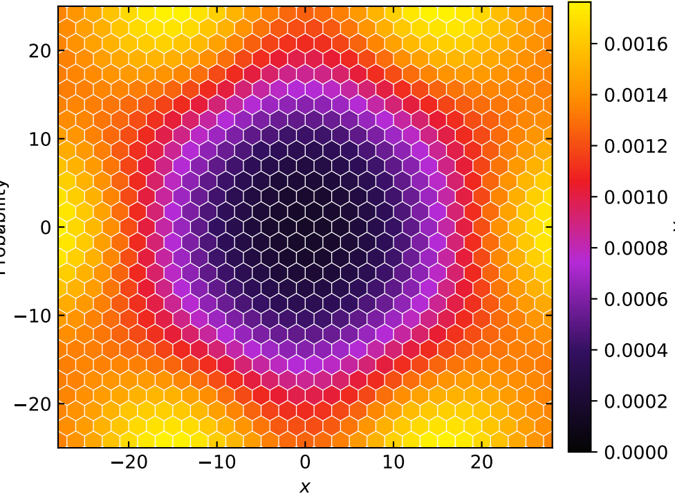
(b) Kinetic Monte Carlo ( N = 100,000,000 )
