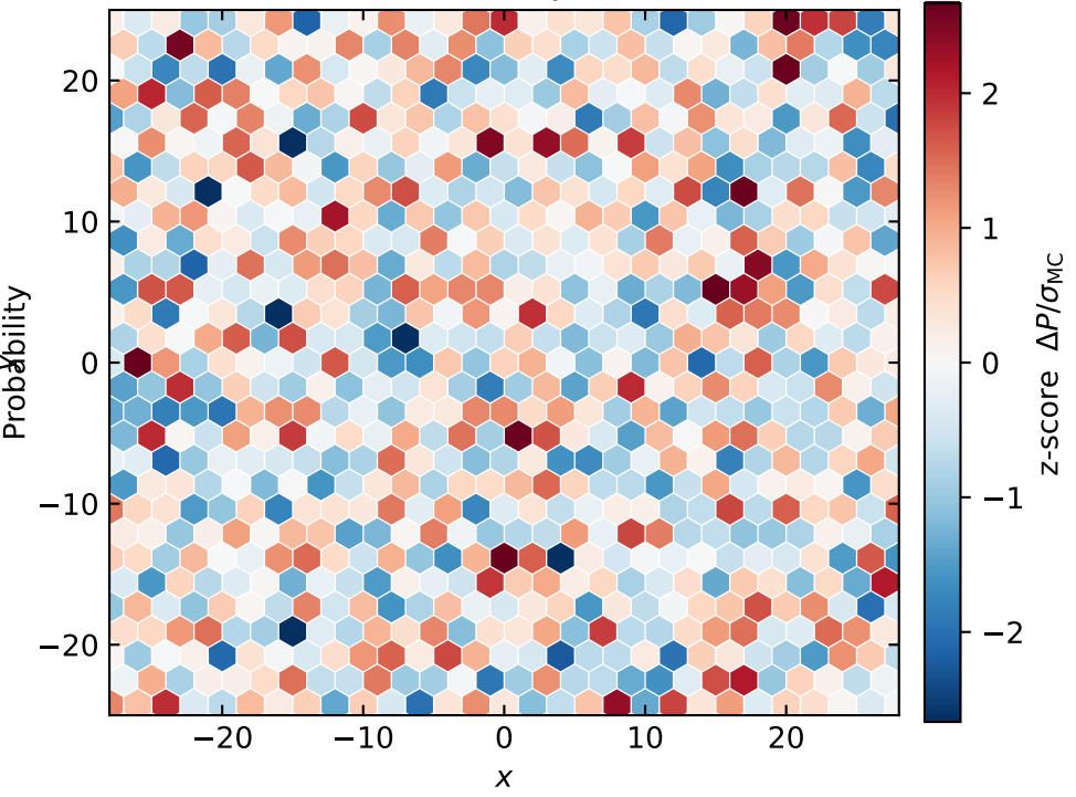
(c) Residual (P_{\text{theory}} - P_{\text{KMC}})/\sigma_{\text{MC}}
