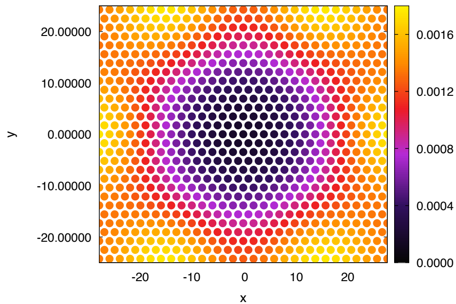
(a) Corrected exact theory ( \gamma=0.01 , \epsilon=0.15 , t=50 )
