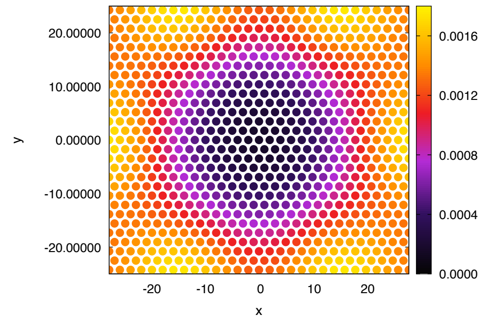
(b) Kinetic Monte Carlo ( N=100,000,000 )
