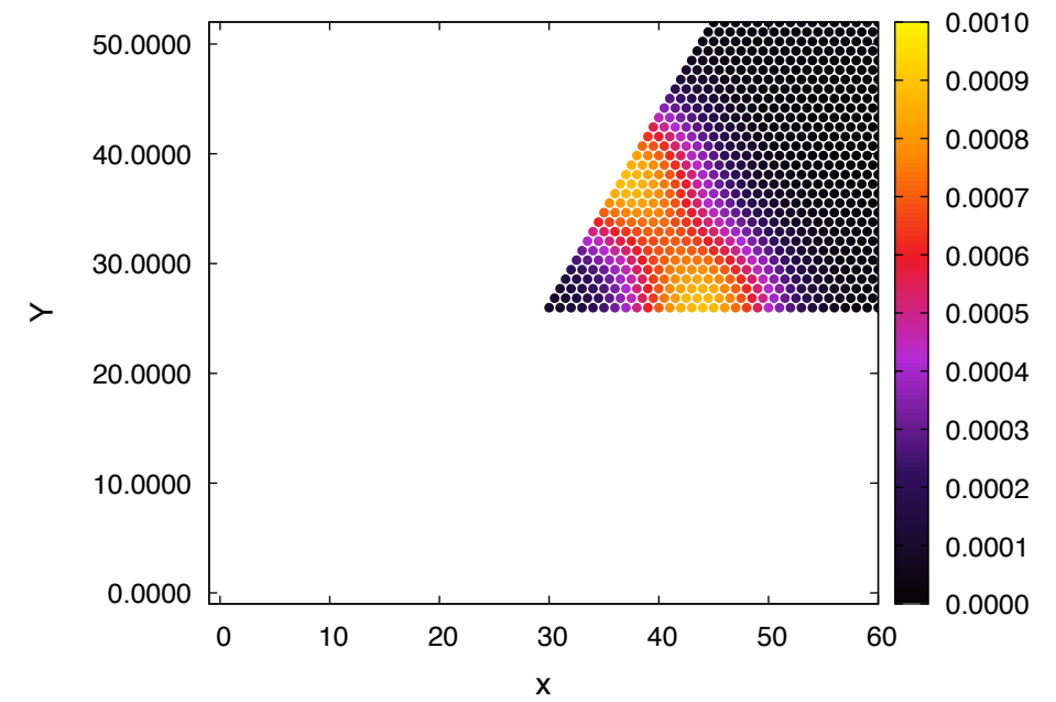
(b) KMC: \gamma=0.01 , \epsilon=0.15 , t=50
