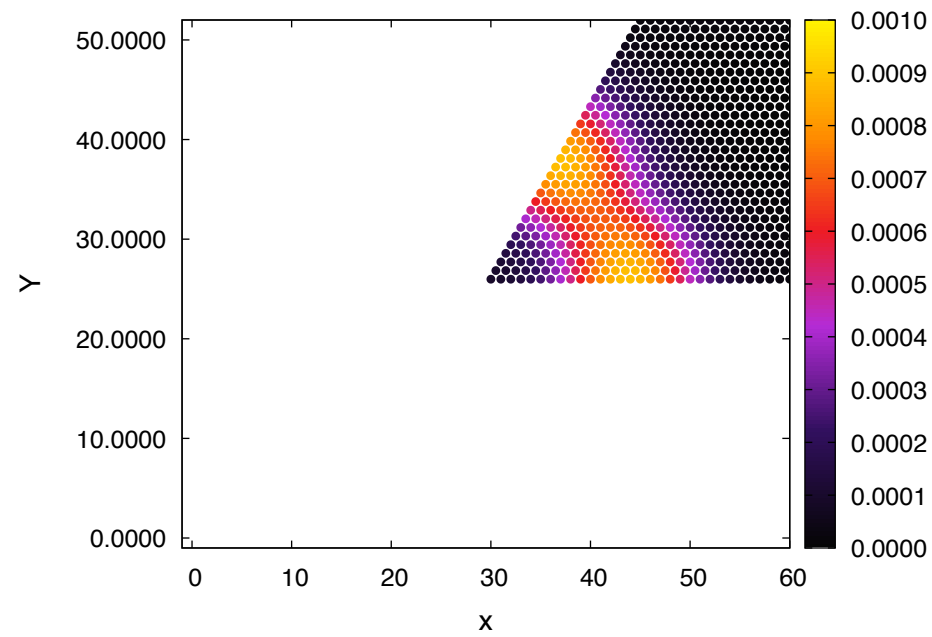
(a) corrected theory: \gamma=0.01 , \epsilon=0.15 , t=50
