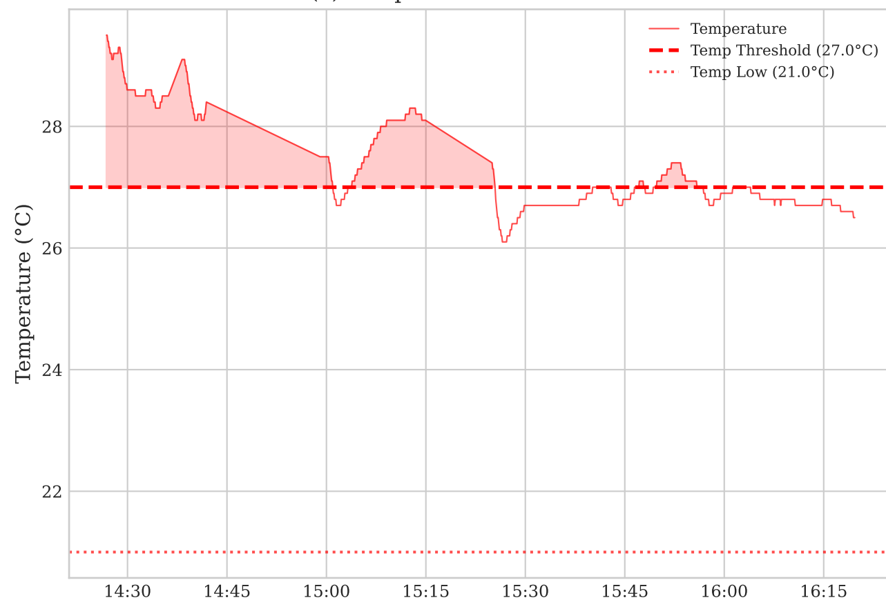
(c) Temperature - MANUAL Mode
