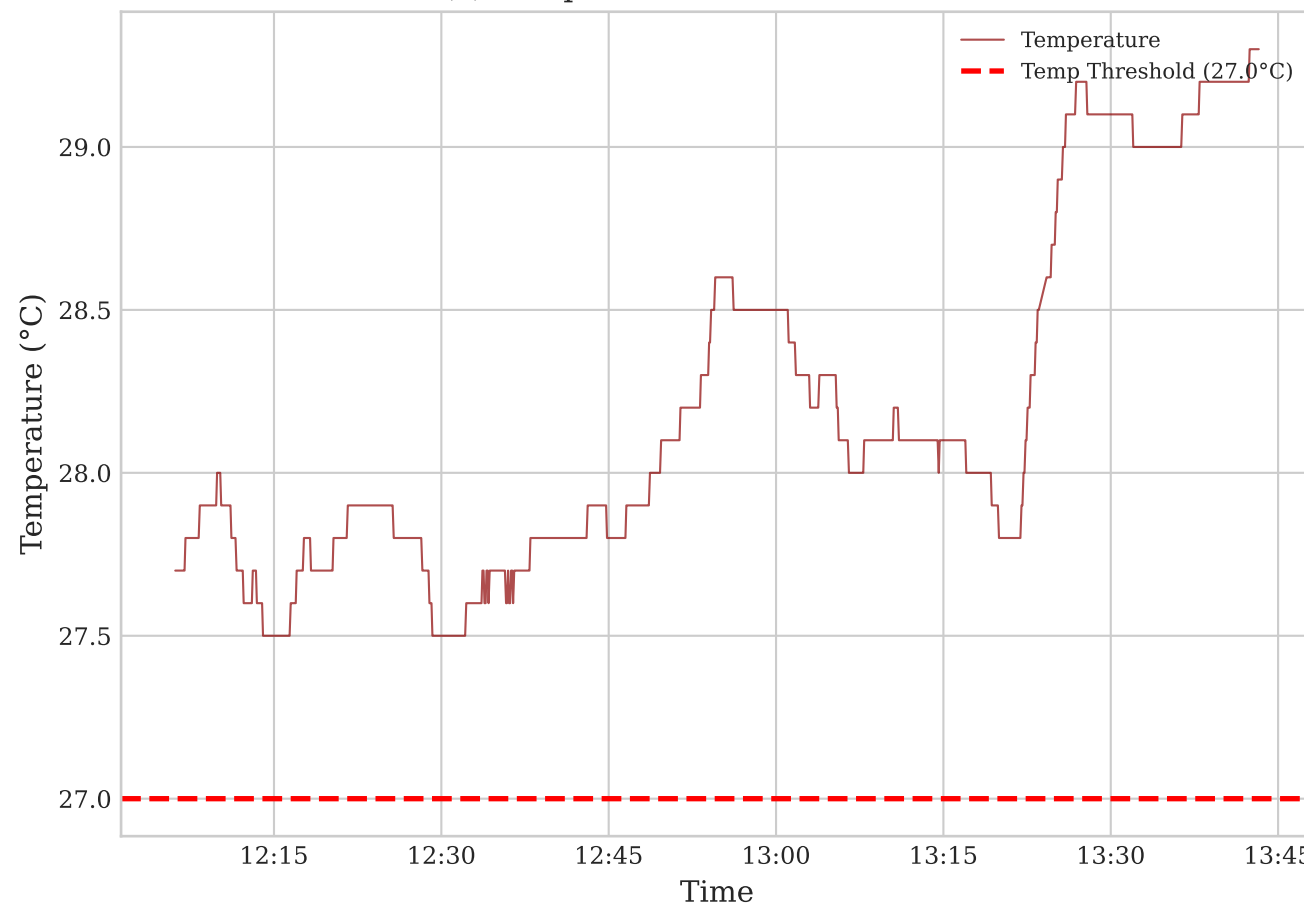
(c) Temperature - MANUAL Mode
