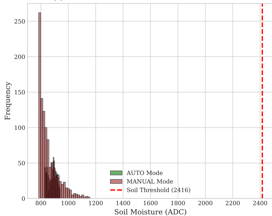
(c) Soil Moisture Distribution: AUTO vs MANUAL
