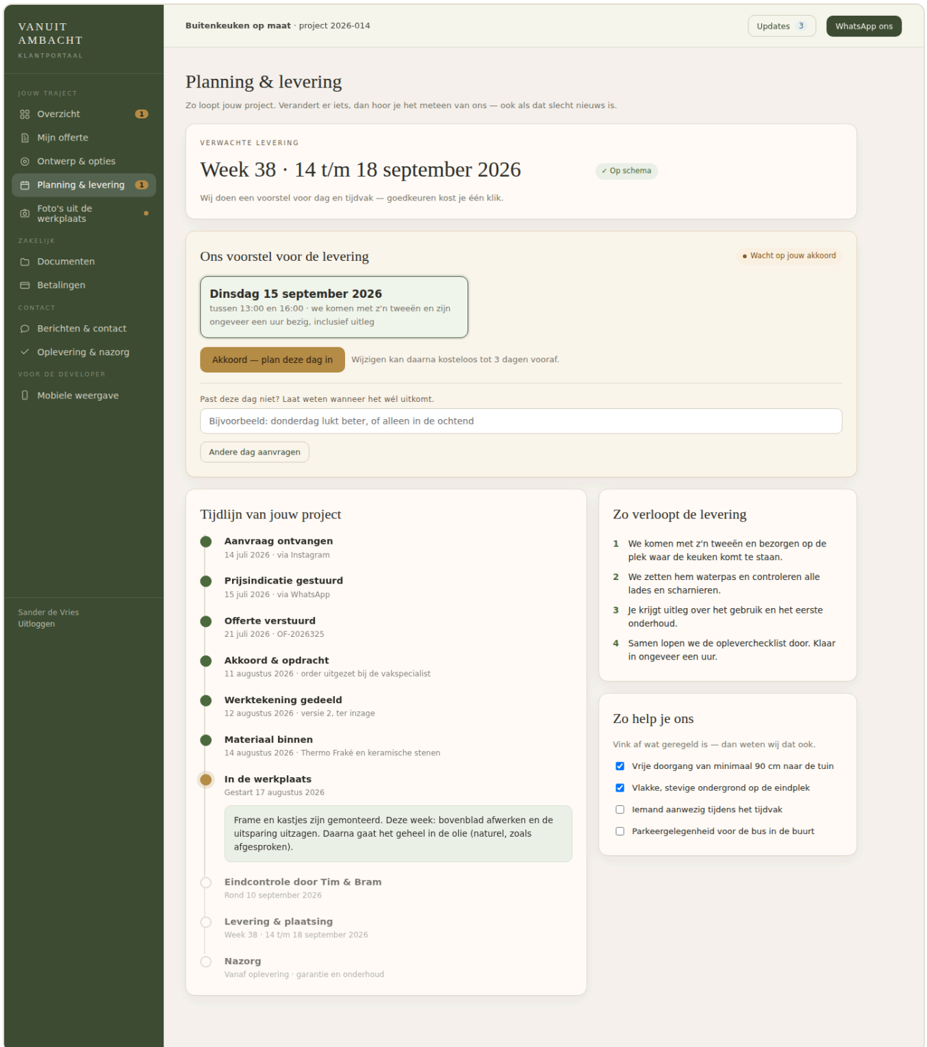
Screen 4 — Schedule & delivery, with the delivery proposal (proposal-approval flow).
