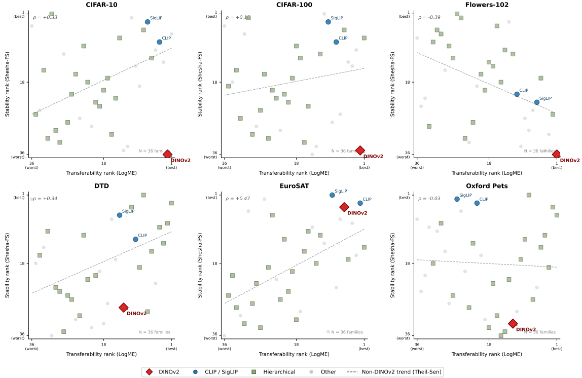
Figure S8: Per-dataset family rankings underlying Figure 4. Each panel plots family-mean transferability rank (LogME) against geometric stability rank (Shesha FS ) for the 36 families, both axes oriented worst to best. DINOv2 occupies the high-transfer, low-stability corner on five datasets, but not on EuroSAT, where it ranks among the most stable families. This is the within-family confirmation of the concentration-stability relationship of Sec. 4.4: EuroSAT is the dataset on which DINOv2’s spectrum is most concentrated. The robust Theil-Sen cross-family trend is positive or null on five datasets (CIFAR-10 +0.33, CIFAR-100 +0.16, DTD +0.34, EuroSAT +0.47, Oxford Pets −0.03) and negative only on Flowers-102 (−0.39), so there is no consistent transferability-stability trade-off across families. Flowers-102, where DINOv2’s own dissociation is sharpest, is the sole dataset that shows one.
