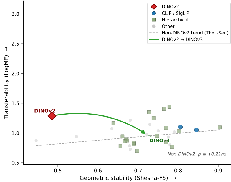
Figure 4: DINOv2 dissociates geometric stability from transferability; the population at large does not. Family-mean transferability (LogME) against geometric stability (Shesha FS ) for 36 architectural families, averaged across the six datasets. DINOv2 (red) is the lone outlier, sitting far to the low-stability side of the population while remaining highly transferable. Across the other 35 families the two quantities are not traded off: the robust Theil-Sen trend is flat to weakly positive ( \rho = +0.21 , not significant), and CLIP and SigLIP combine high stability with competitive transferability, so low stability is not a general cost of transfer. The arrow marks the generational change from DINOv2 to DINOv3, which under Gram anchoring returns from the outlier position onto the population trend. The per-dataset breakdown, including the EuroSAT exception where DINOv2 is itself highly stable, is given in Appendix S8.
