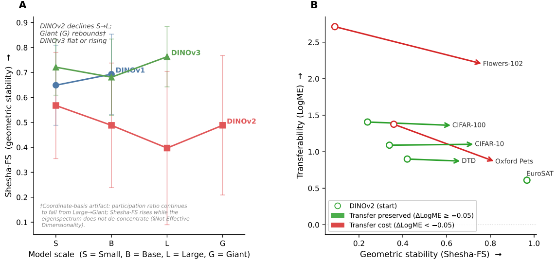
Figure 5: Gram anchoring closes the DINOv2 dissociation. A. Geometric stability ( \text{Shesha}_{\text{FS}} ) against model scale, mean \pm SD across the six datasets. DINOv2 stability falls from small to large; the apparent rebound at giant is a coordinate-basis artifact, since the participation ratio keeps falling from large to giant and the eigenspectrum does not de-concentrate (Sec. 4.4). DINOv3 stays flat or rises, and DINOv1 (small and base only) sits above DINOv2 throughout, so the dissociation tracks the training objective rather than model scale. B. Matched at the large scale, the change from DINOv2 to DINOv3 on the stability-transfer plane, one arrow per dataset. On four of six datasets DINOv3 gains stability with transfer preserved ( \Delta\text{LogME} \geq -0.05 , green); on Flowers-102 and Oxford Pets the stability gain carries a transfer cost (red). EuroSAT shows no arrow because both generations are already highly stable there.
