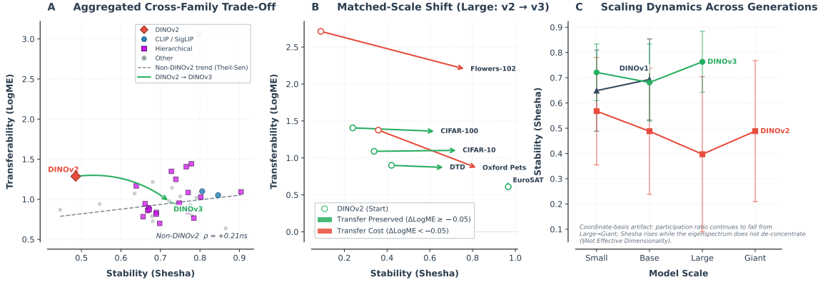
Figure 5: A. DINOv2 dissociates geometric stability from transferability; the population at large does not. Family-mean transferability ( \text{LogME} ) against geometric stability ( \text{Shesha}_{\text{FS}} ) for 36 architectural families, averaged across the six datasets. DINOv2 (red) is the lone outlier, sitting far to the low-stability side of the population while remaining highly transferable. Across the other 35 families the two quantities are not traded off: the robust Theil-Sen trend is flat to weakly positive ( \rho = +0.21 , not significant), and CLIP and SigLIP combine high stability with competitive transferability, so low stability is not a general cost of transfer. The arrow marks the generational change from DINOv2 to DINOv3, which under Gram anchoring returns from the outlier position onto the population trend. The per-dataset breakdown, including the EuroSAT exception where DINOv2 is itself highly stable, is given in Appendix S8. B. Matched at the large scale, the change from DINOv2 to DINOv3 on the stability-transfer plane, one arrow per dataset. On four of six datasets DINOv3 gains stability with transfer preserved ( \Delta\text{LogME} \geq -0.05 , green); on Flowers-102 and Oxford Pets the stability gain carries a transfer cost (red). EuroSAT shows no arrow because both generations are already highly stable there. C. Geometric stability ( \text{Shesha}_{\text{FS}} ) against model scale, mean \pm SD across the six datasets. DINOv2 stability falls from small to large; the apparent rebound at giant is a coordinate-basis artifact, since the participation ratio keeps falling from large to giant and the eigenspectrum does not de-concentrate (Sec. 4.4). DINOv3 stays flat or rises, and DINOv1 (small and base only) sits above DINOv2 throughout, so the dissociation tracks the training objective rather than model scale.
