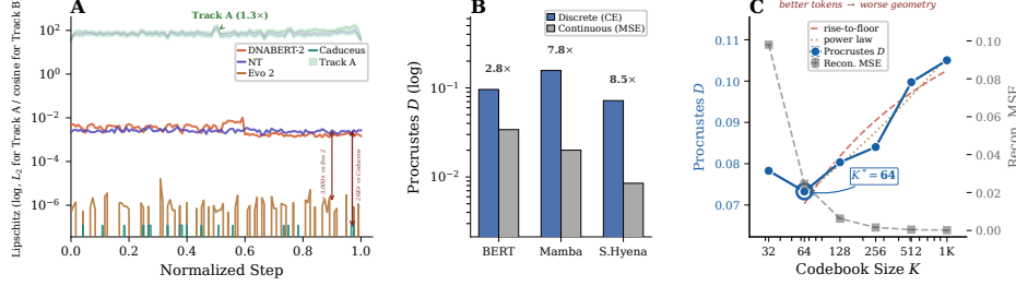
Figure 1: A. Track A vs. Track B Lipschitz profiles: smooth arcs (continuous physics) vs. divergent, multi-scale fracture (discrete biology). Track A uses L_2 Lipschitz and Track B uses cosine Lipschitz (dimension-invariant across embedding sizes), so only within-track spreads are comparable: 1.3\times within Track A, \sim 3,000\times within Track B. B. Continuous vs. discrete Procrustes D across architectures on the Lorenz dataset at 1% noise. All continuous conditions cluster near zero; discrete conditions span an order of magnitude. C. VQ double bind on the Lorenz attractor at 1% noise: reconstruction MSE (decreasing) vs. Procrustes D (non-monotone) vs. codebook size K . Both candidate slow-growth fits are shown on the ascending branch ( K \geq K^* ): rise-to-floor ( D = B - A/\log K ) and a weak power law ( D \propto K^{0.13} ). We do not adjudicate between them. Better tokens improve reconstruction while worsening geometry.
