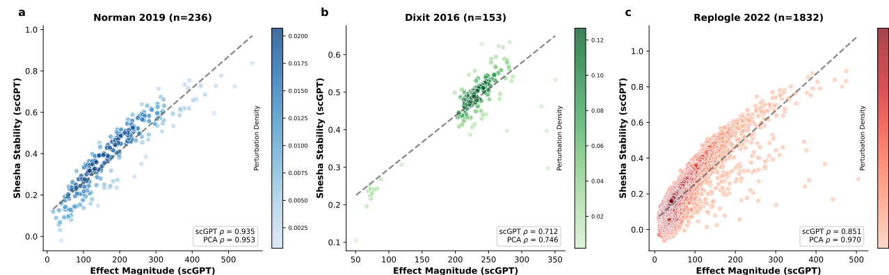
Figure 4: The magnitude-stability relationship persists in nonlinear foundation model embeddings Effect magnitude (x-axis) vs perturbation stability (y-axis) computed in scGPT “Whole Human” embeddings for three datasets: (a) Norman 2019 ( n = 236 , scGPT \rho = 0.935 , PCA \rho = 0.953 ), (b) Dixit 2016 ( n = 153 , scGPT \rho = 0.712 , PCA \rho = 0.746 ), (c) Replogle 2022 ( n = 1,832 , scGPT \rho = 0.851 , PCA \rho = 0.970 ). Dashed lines: linear regression. The dataset rank order is preserved across embedding methods (Norman > Replogle > Dixit). scGPT correlations are consistently slightly lower than PCA, consistent with the nonlinear embedding resolving additional manifold structure that PCA collapses. The largest drop occurs in Replogle, the most diverse screen.
