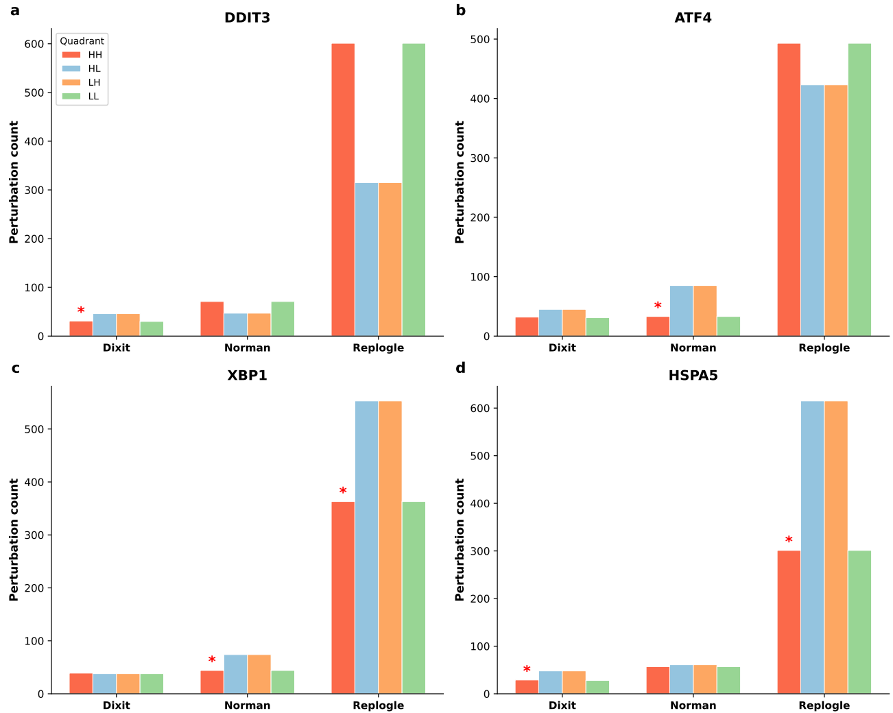
Supplementary Figure S12: Quadrant depletion analysis of stability versus stress. Perturbations split at median stability and median stress expression (dashed lines). Quadrant counts annotated. The high-stability/high-stress (HH) quadrant is systematically depleted across multiple stress markers and datasets (Fisher's exact test; Table S20), supporting the interpretation that geometric coherence is a prerequisite for cellular homeostasis. Perturbations producing incoherent cellular responses (low stability) are more likely to induce elevated stress signatures.
