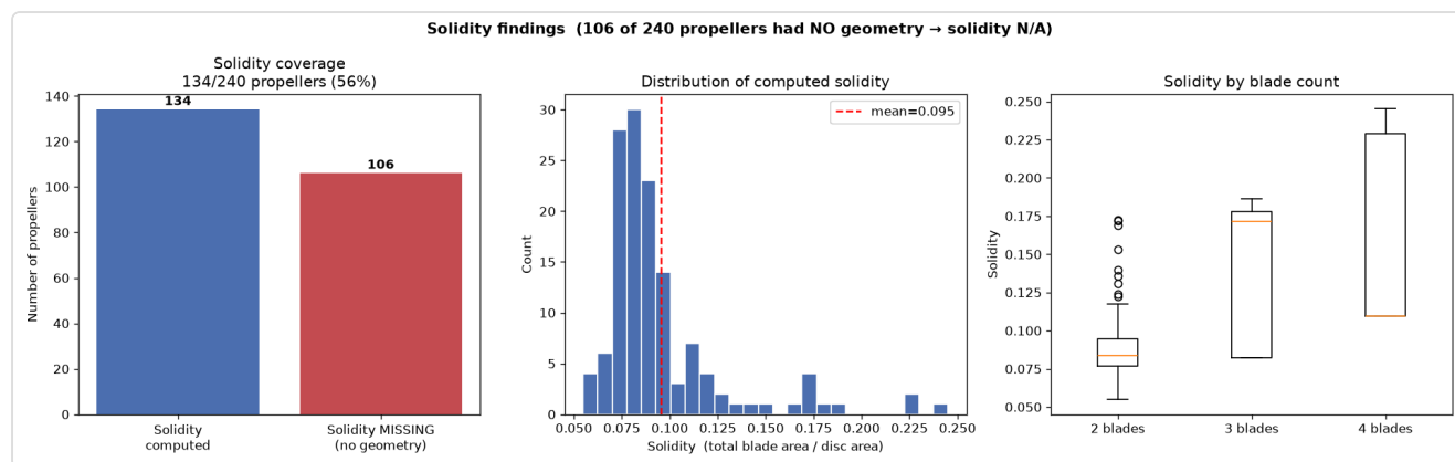
Figure — 01_solidity_findings.png
