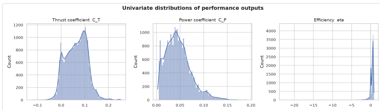
Figure — 02_target_distributions.png
