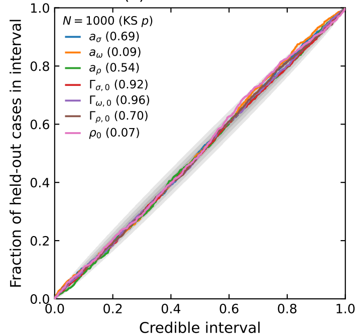
(a) Nucleonic A-NET
