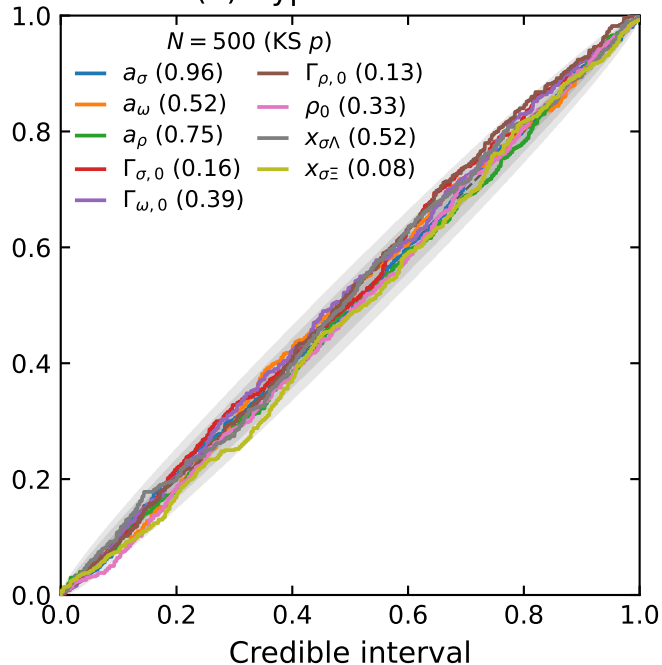
(b) Hyperonic A-NET
