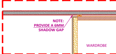
D)DETAIL-B
