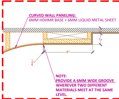
C)DETAIL-A
