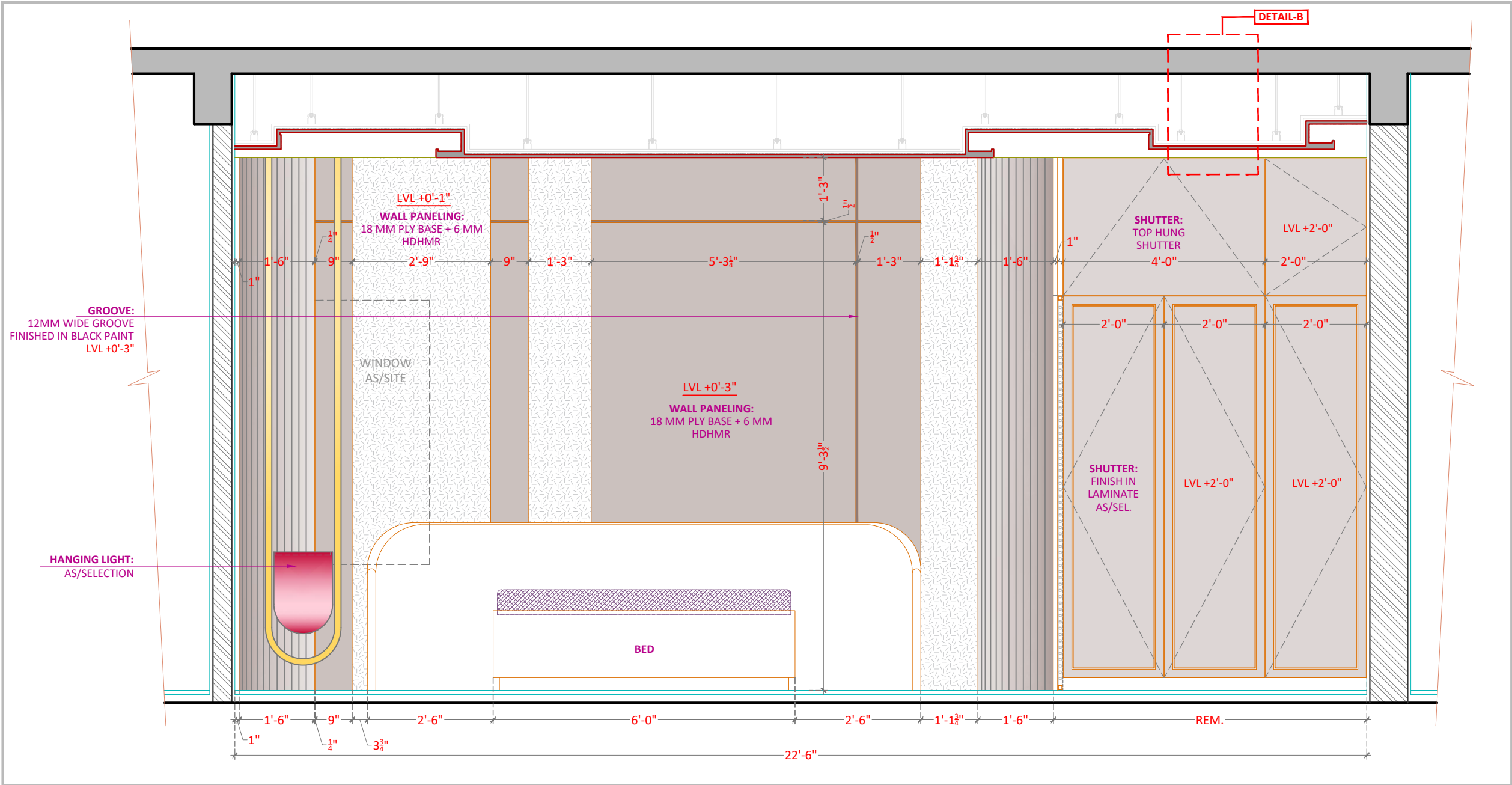
B)WORKING ELEVATION
