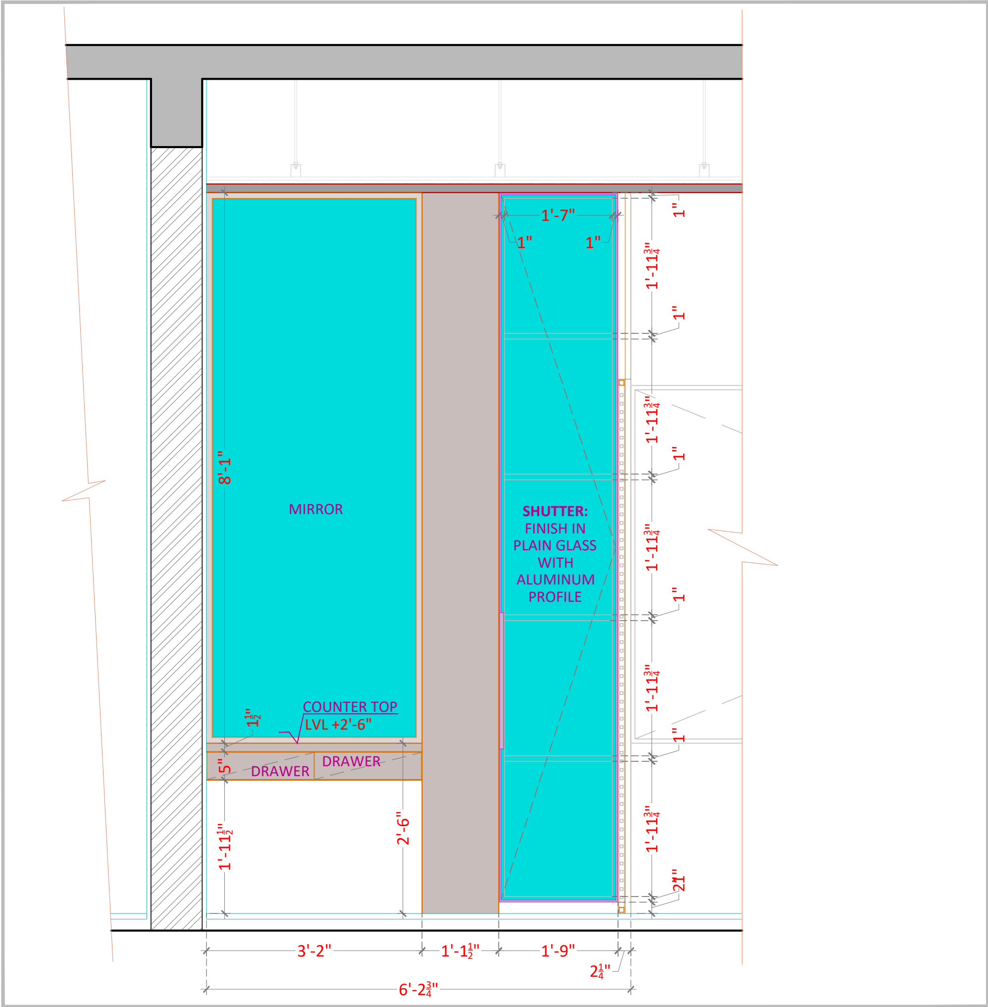
B) WORKING ELEVATION
