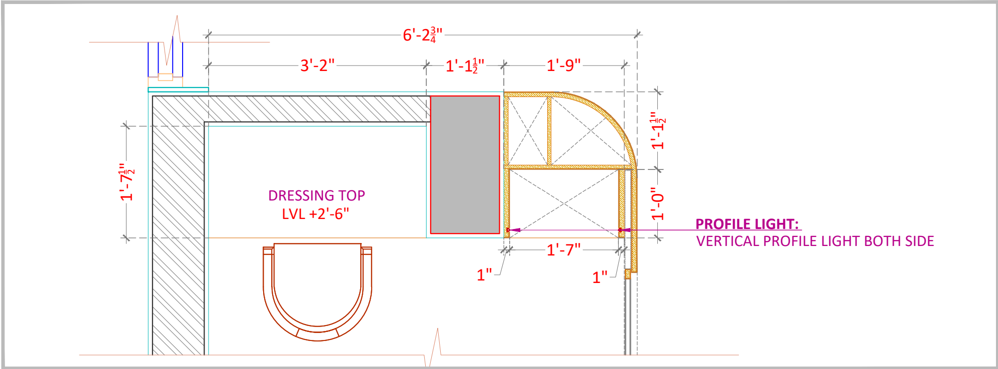
A) WORKING PLAN
