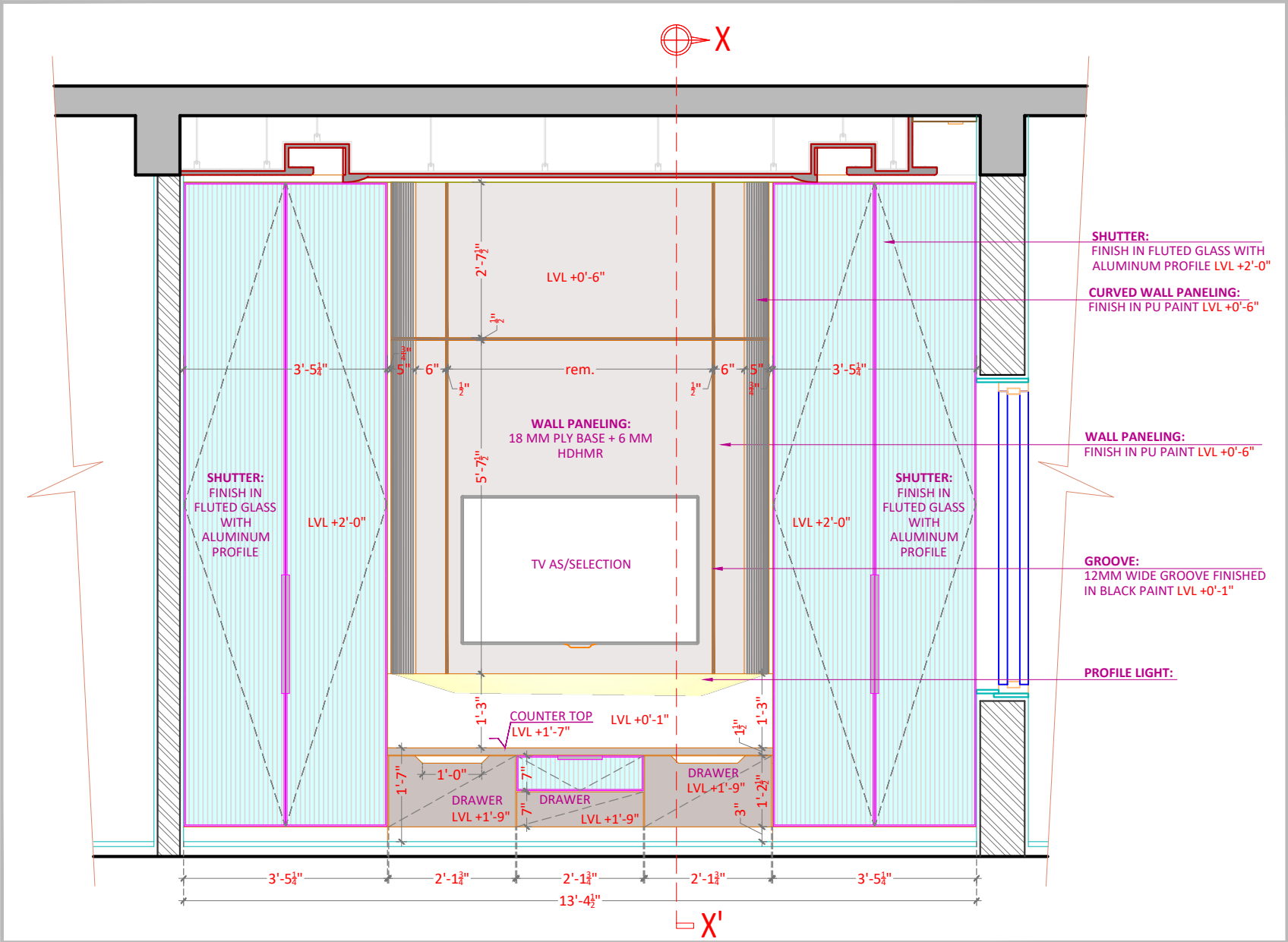
B)WORKING ELEVATION
