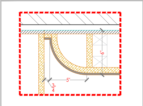
F)DETAIL - B
