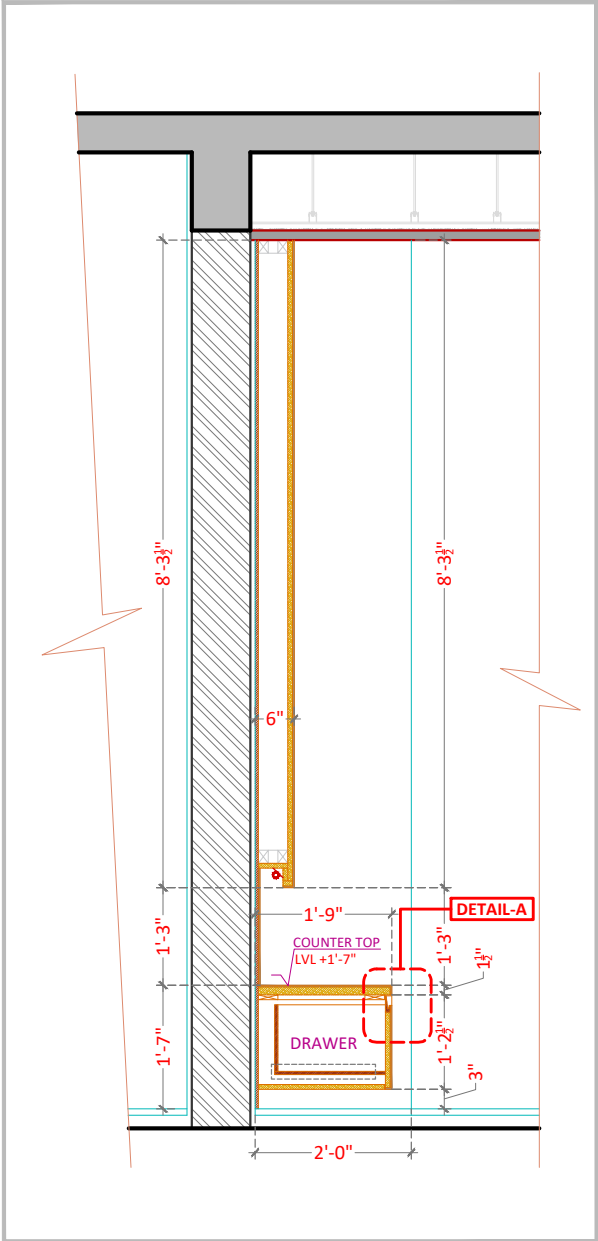
D)SECTION X - X'
