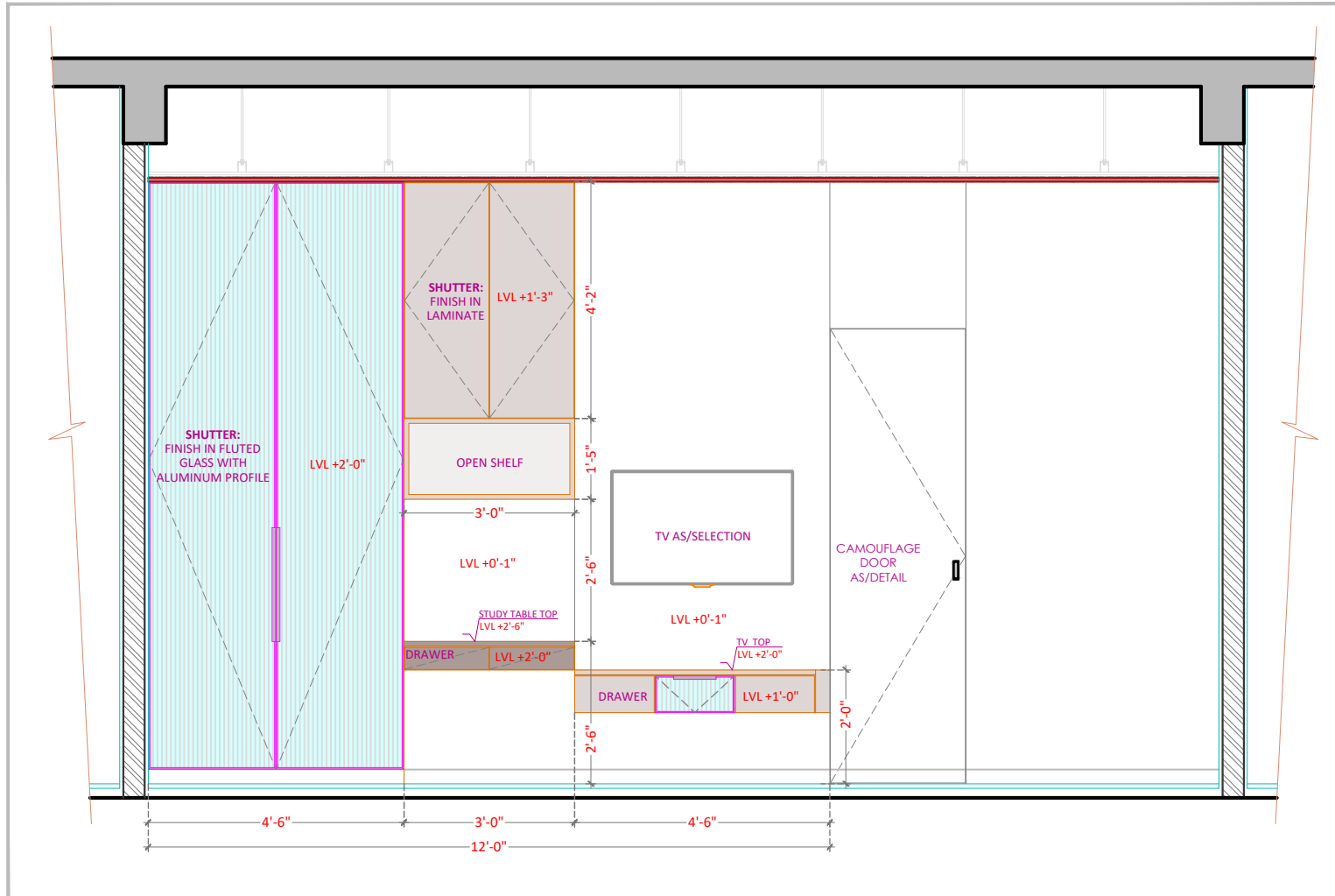
C)WORKING ELEVATION - C
