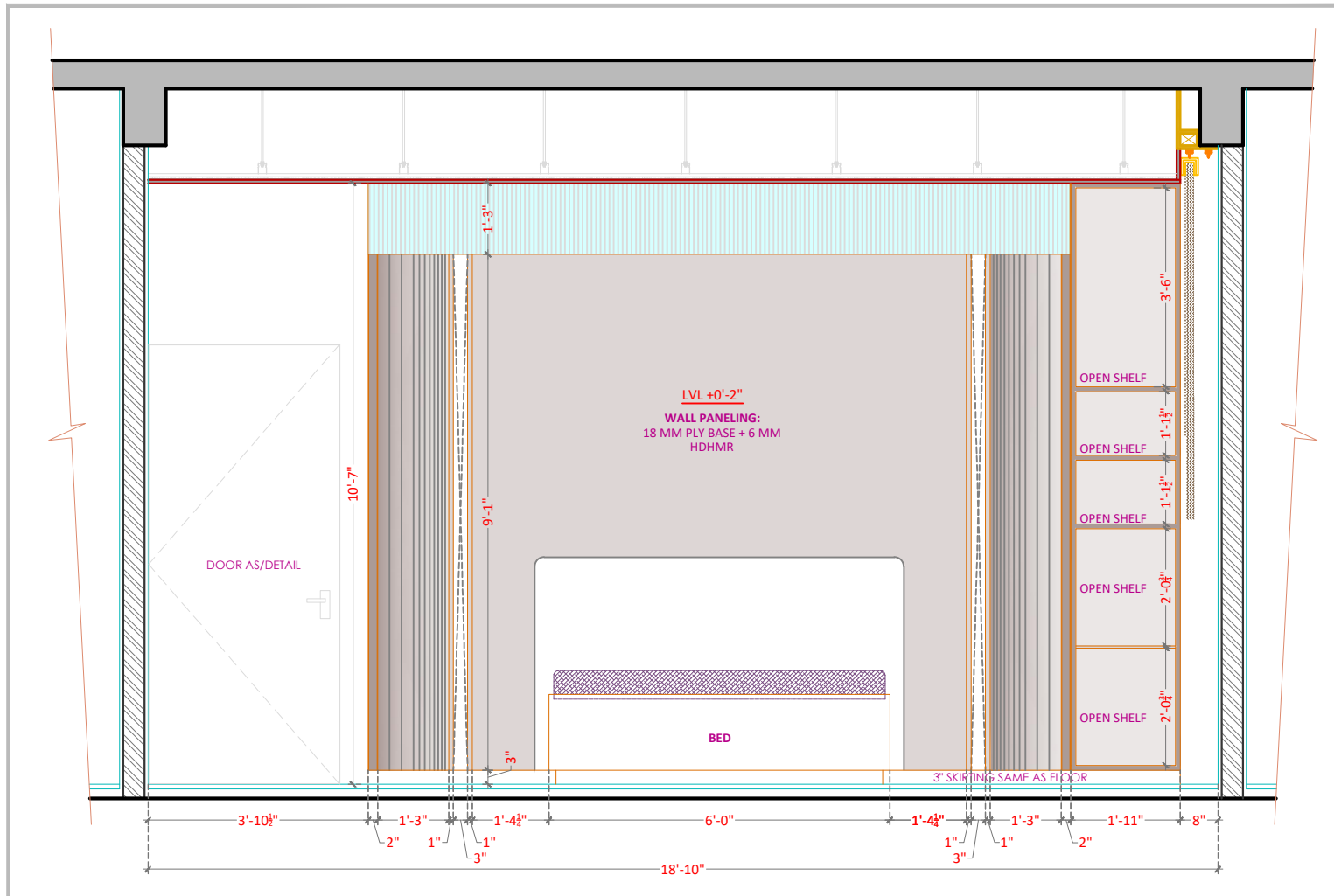
A)WORKING ELEVATION - A
