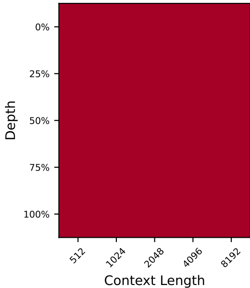
Learned Absolute
