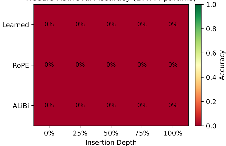
Needle Retrieval Accuracy (17.7M params)
