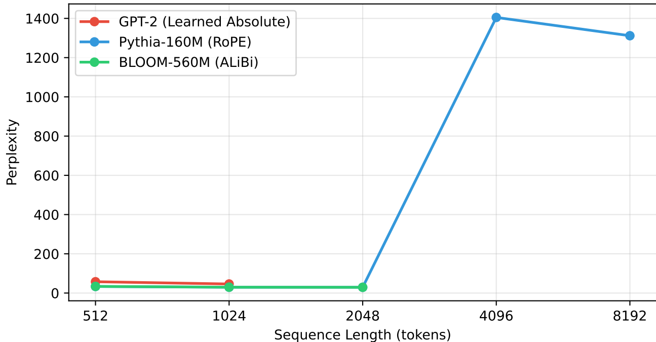
Zero-Shot Perplexity vs. Sequence Length
