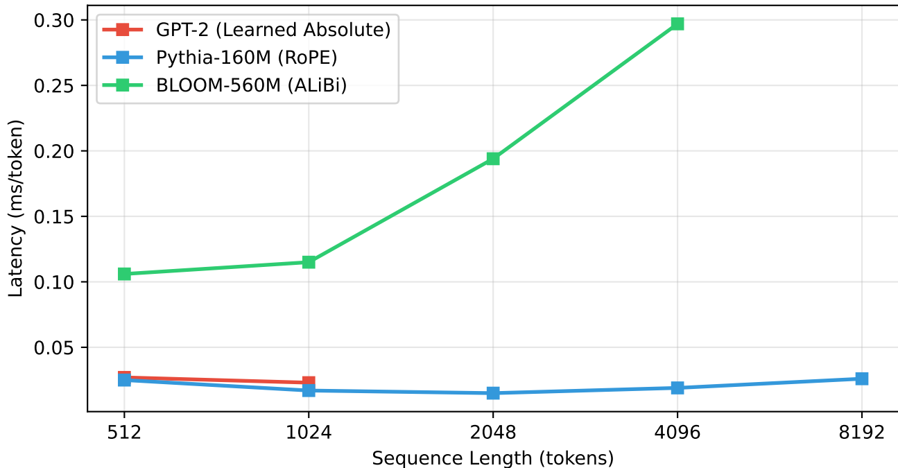
Inference Latency vs. Sequence Length
