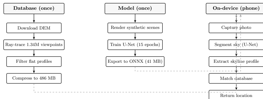
Figure 4-1. Pipeline overview.
