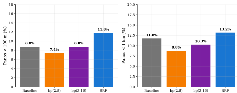
Figure 6-6. Per-scorer accuracy.
