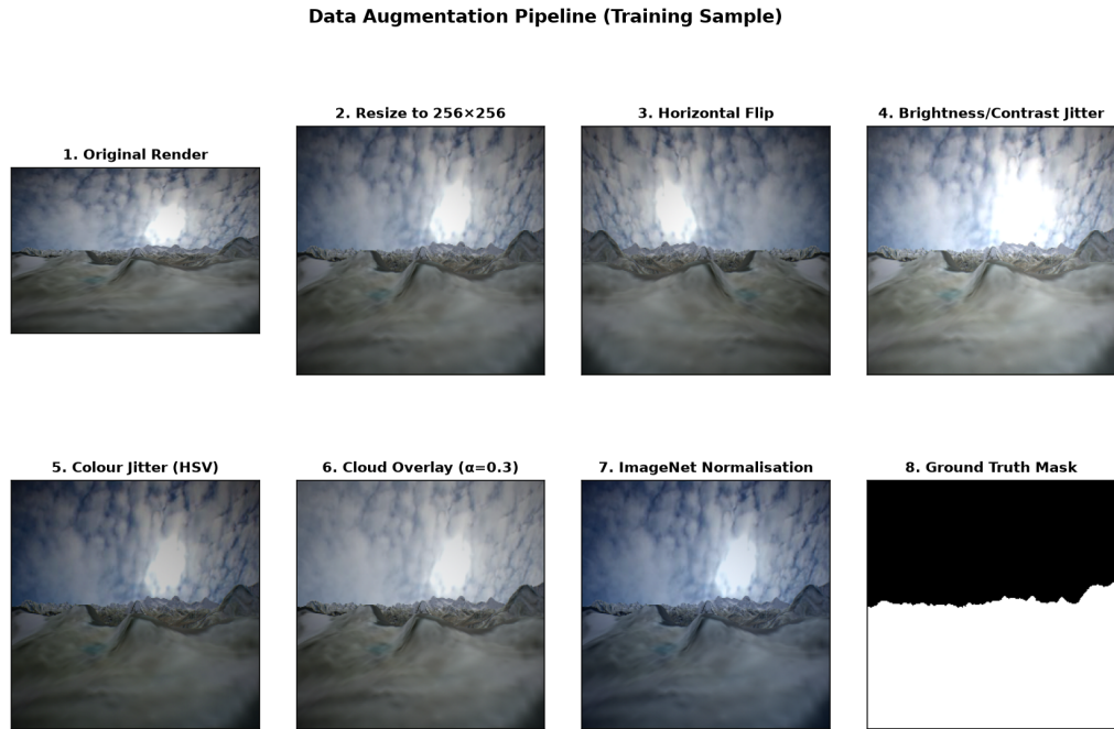
Figure 4-5. Augmentation pipeline.
