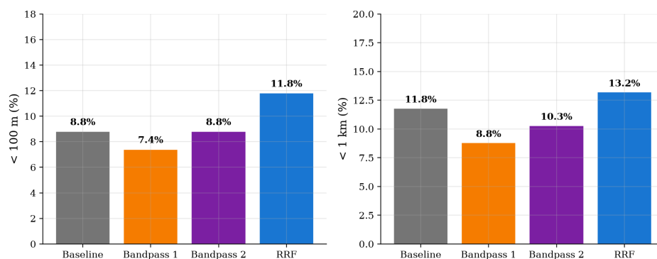
Figure 6-5. Per-scorer accuracy.
