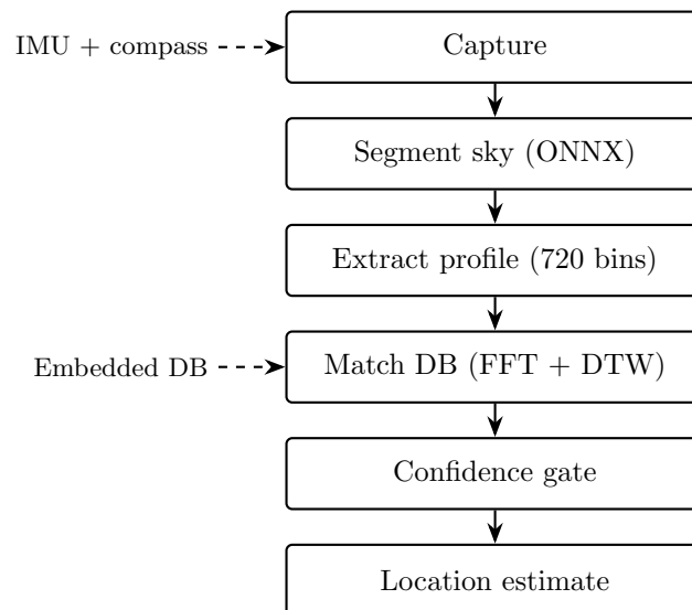
Figure 4-6. Mobile-side pipeline.
