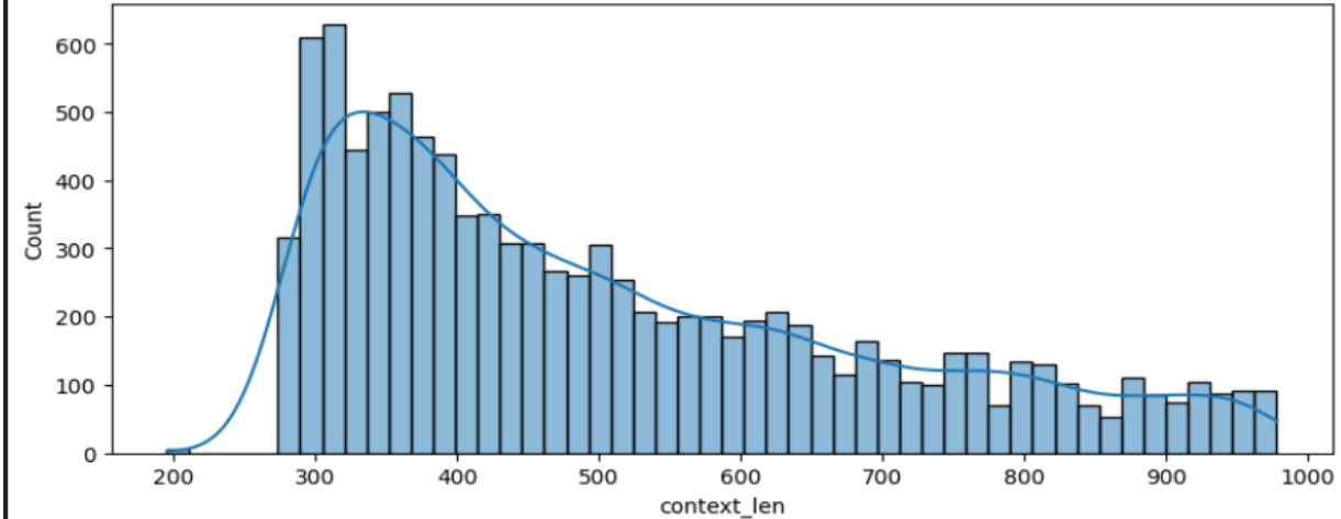
CMRC: Context length distribution (chars)
