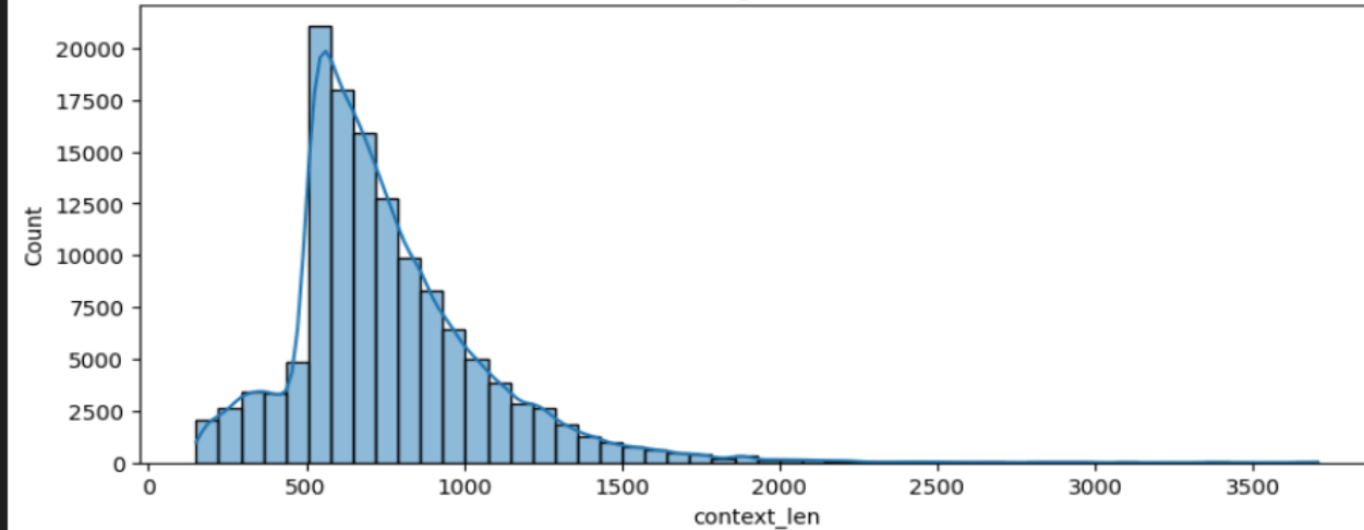
SQuAD: Context length distribution (chars)
