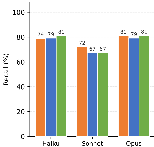
Recall
