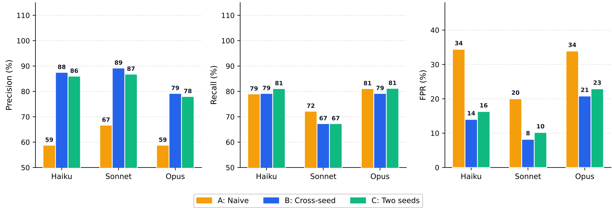
MORPH-DA under three evaluation conditions
