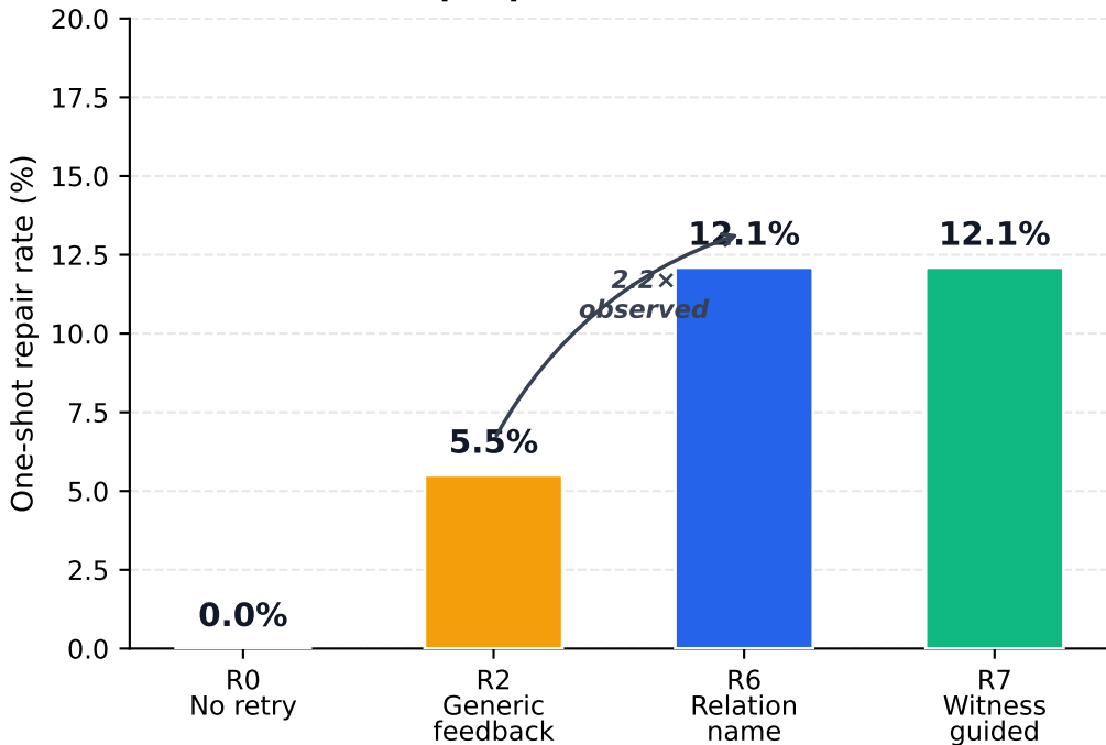
One-step repair success rate (n=91)
