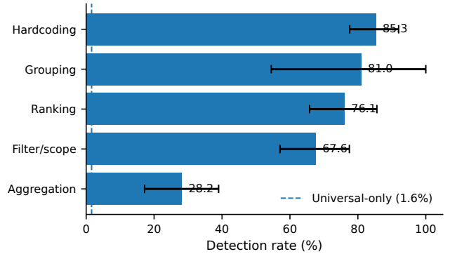
Figure 2: Mutation detection by fault family. Aggregation is hardest because a wrong aggregation can preserve the winning label on ranking tasks. Error bars are task-clustered 95% bootstrap intervals.
