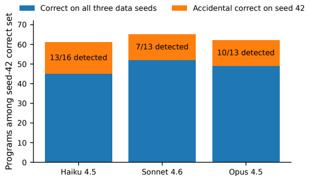
Figure 3: Programs correct on seed 42 split into truly correct and accidental correct after fixed-program re-execution on seeds 7 and 123.
