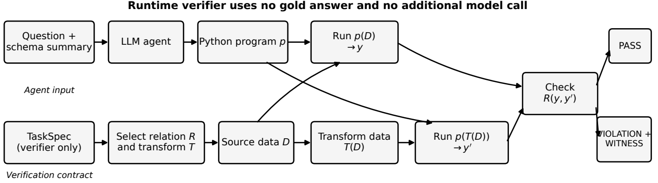
Figure 1: MORPH-DA separates program generation from verification. The agent receives only the question and schema summary. The verifier receives the candidate program and a structured task specification, generates deterministic follow-up tables, re-executes the unchanged program, and checks the expected output relation. No gold answer or additional LLM call is used during verification.
