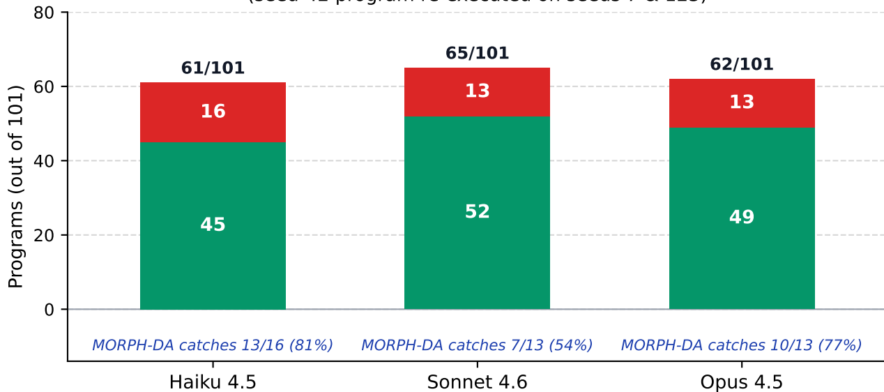
Accidental Corrects by Model (seed-42 program re-executed on seeds 7 & 123)
