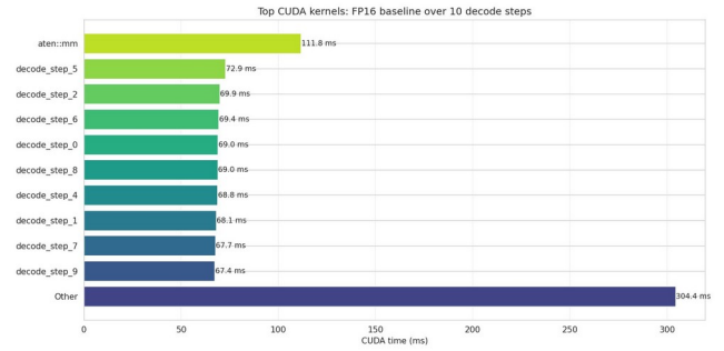
Fig. 5. PyTorch profiler kernel breakdown for 10 FP16 decode steps. aten::mm dominates at 111.8 ms, with the rest spread across many smaller operations for layer normalization, softmax, and elementwise operations.
