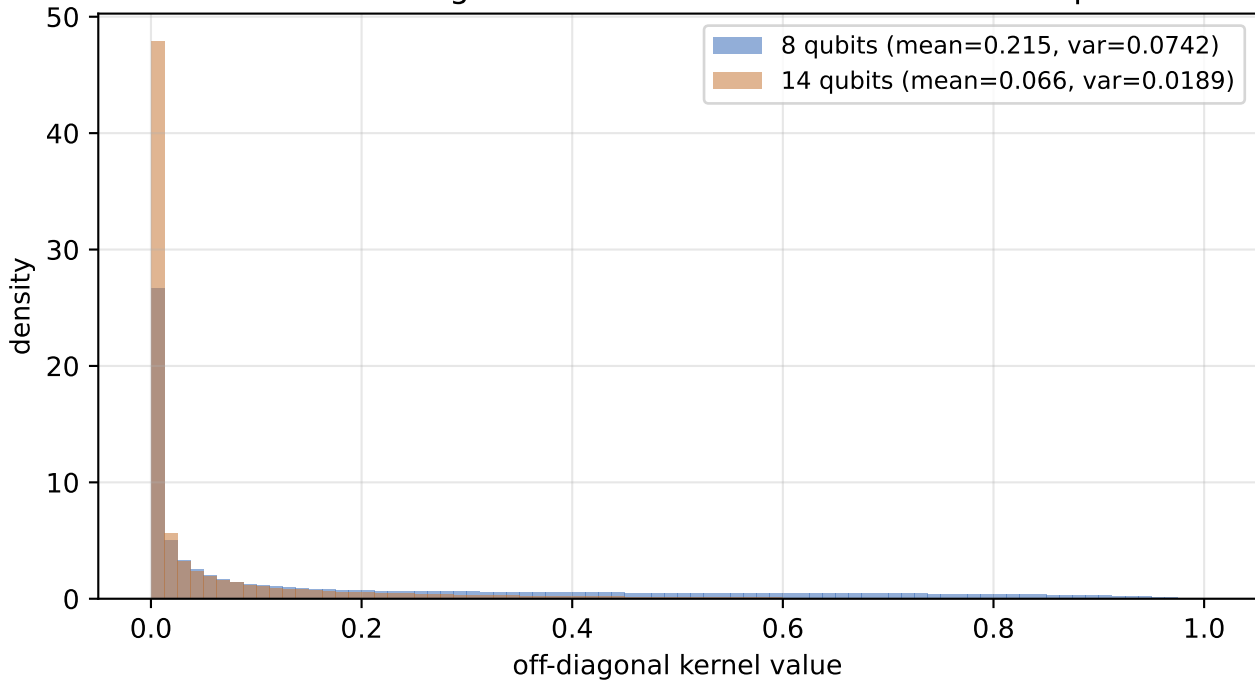
BSCM-uniform off-diagonal distribution: concentration with qubit count
