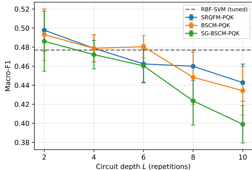
So2Sat (17 classes)
