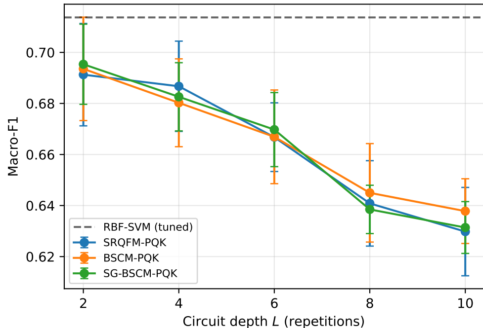
EuroSAT (10 classes)
