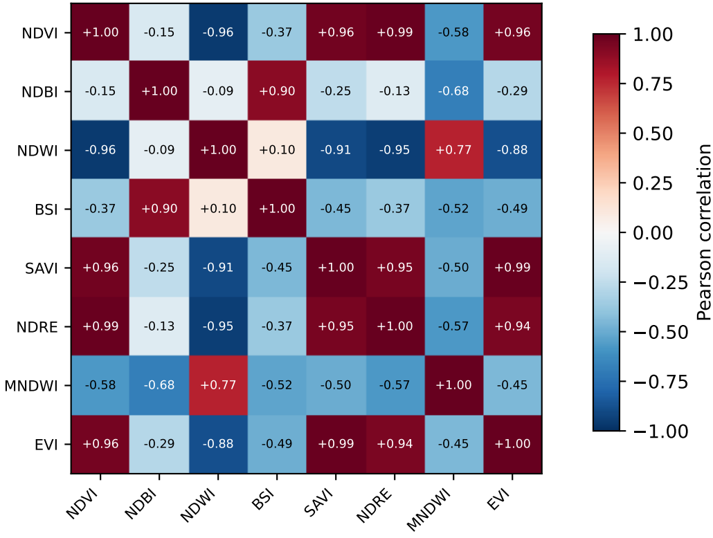
EuroSAT physics-8 (Pearson \rho )
