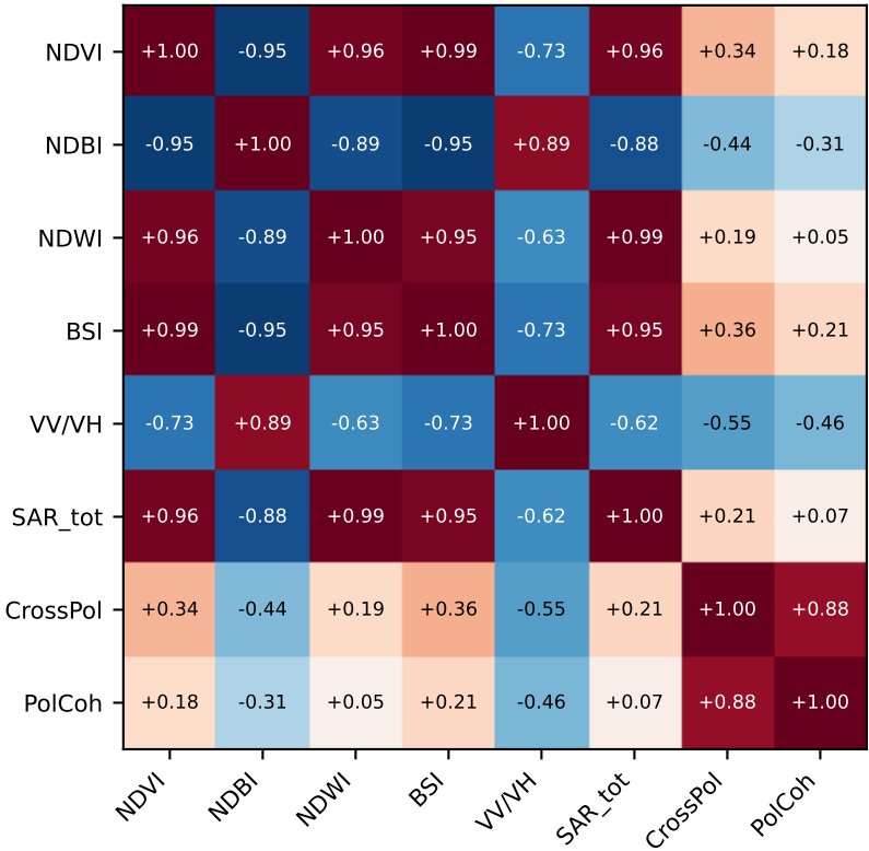
So2Sat physics-8 (Pearson \rho )
